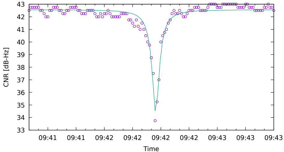
CNR fit for G01 on XiaomiMi8 - drive 2 (DOY263)
