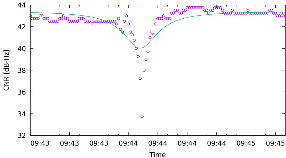
CNR fit for G01 on XiaomiMi8 - drive 3 (DOY263)
