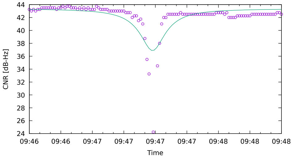
CNR fit for G01 on XiaomiMi8 - drive 5 (DOY263)
