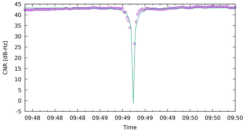
CNR fit for G01 on XiaomiMi8 - drive 6 (DOY263)
