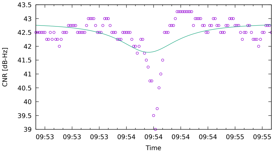
CNR fit for G01 on XiaomiMi8 - drive 9 (DOY263)
