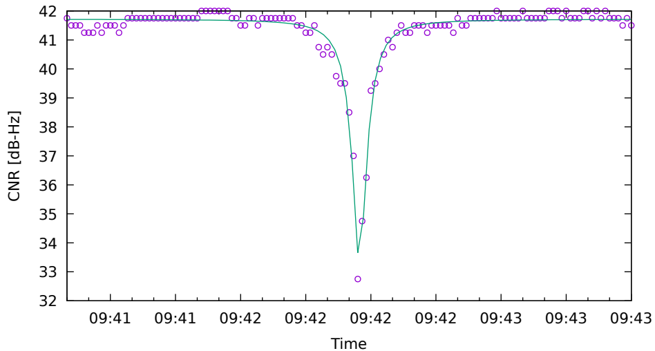
CNR fit for G03 on XiaomiMi8 - drive 2 (DOY263)
