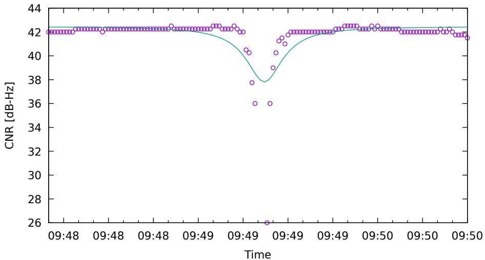
CNR fit for G03 on XiaomiMi8 - drive 6 (DOY263)
