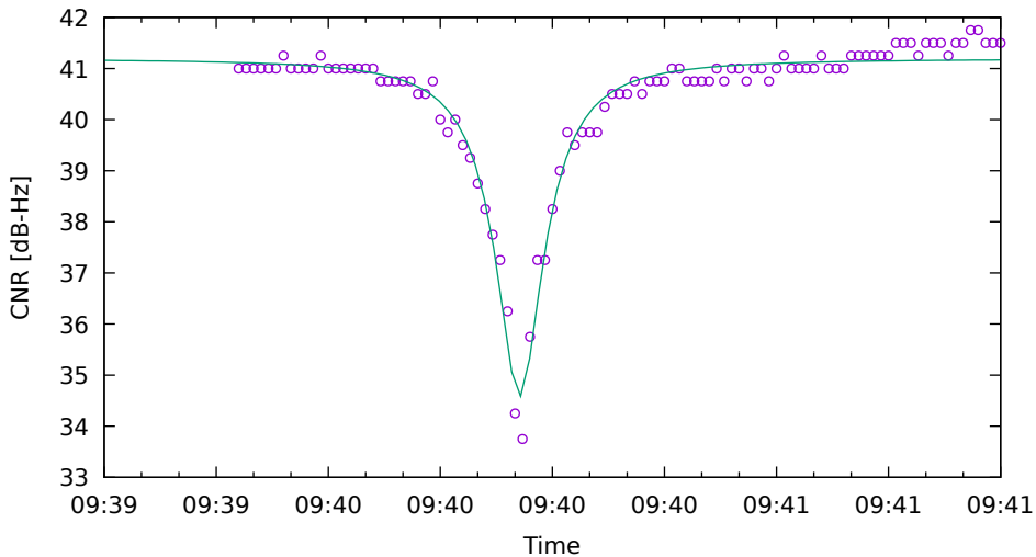
CNR fit for G08 on XiaomiMi8 - drive 1 (DOY263)
