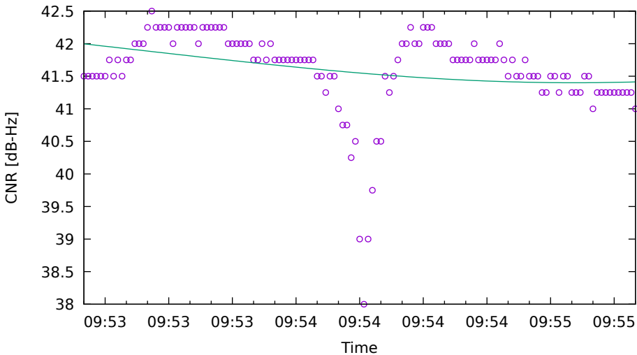
CNR fit for G17 on XiaomiMi8 - drive 9 (DOY263)
