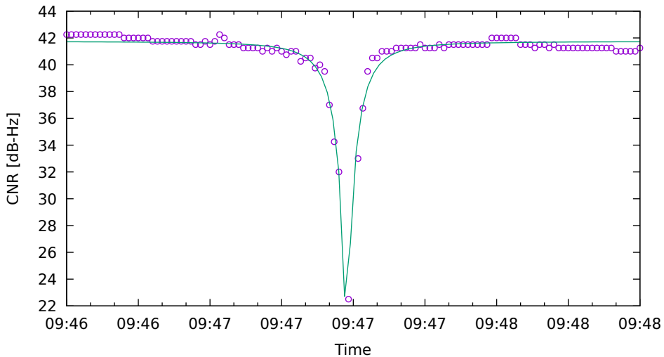
CNR fit for G19 on XiaomiMi8 - drive 5 (DOY263)
