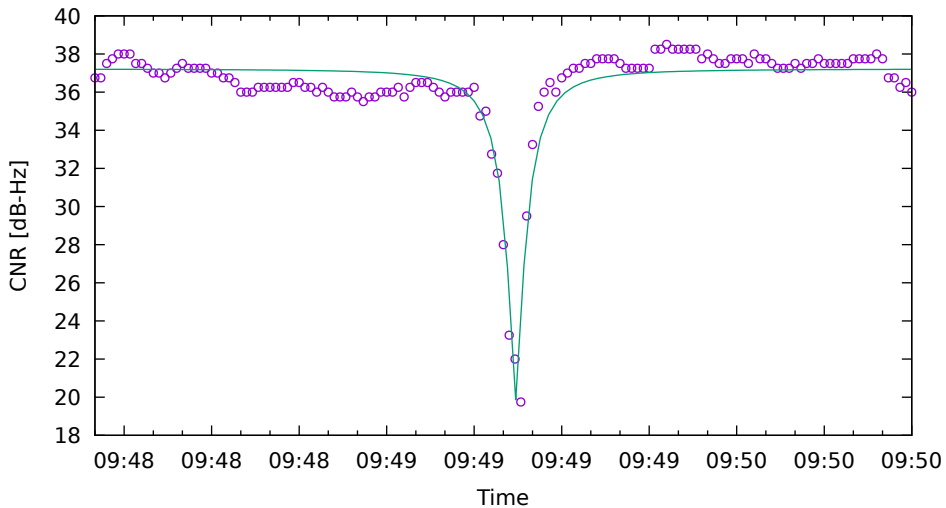
CNR fit for G21 on XiaomiMi8 - drive 6 (DOY263)
