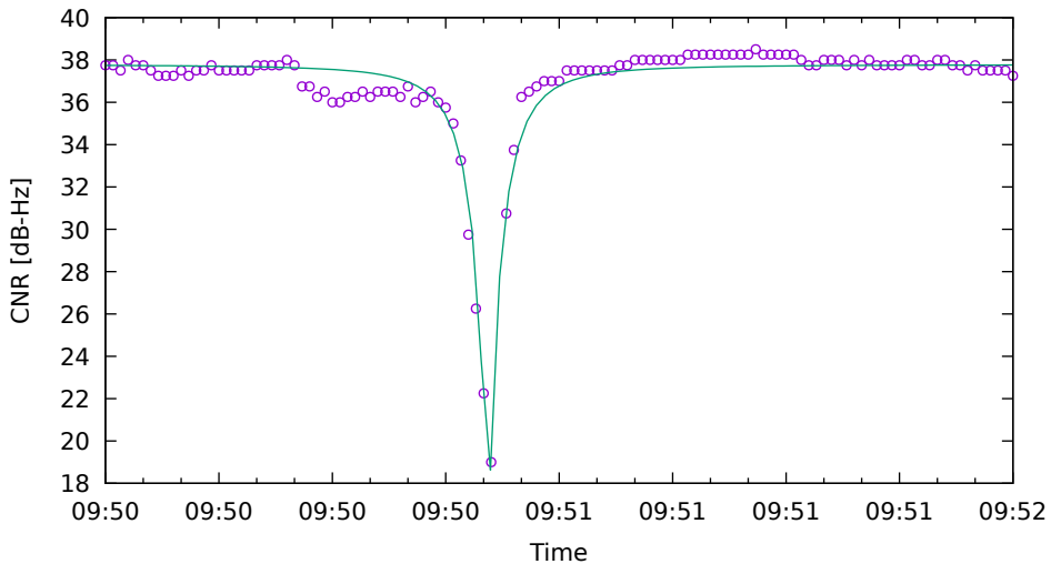
CNR fit for G21 on XiaomiMi8 - drive 7 (DOY263)
