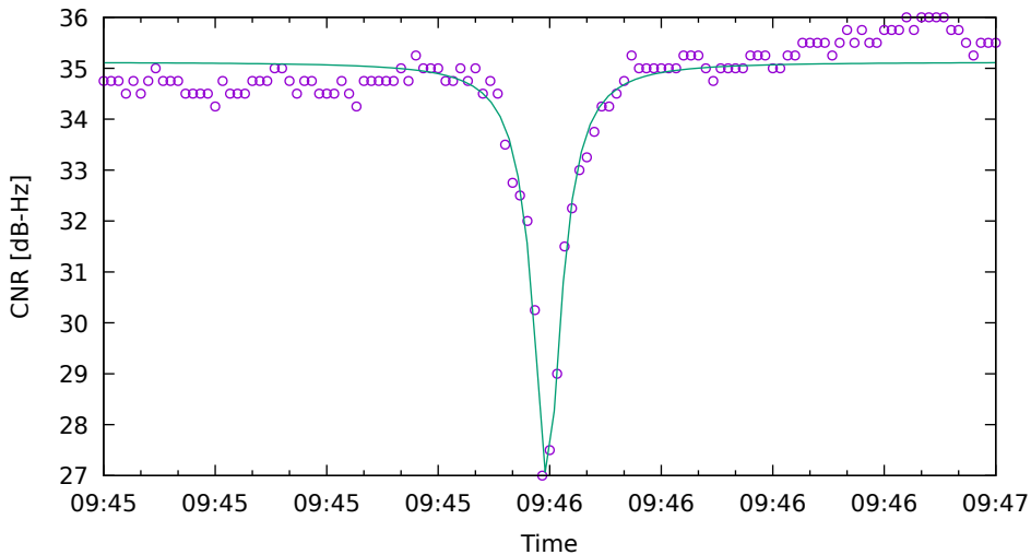
CNR fit for G22 on XiaomiMi8 - drive 4 (DOY263)
