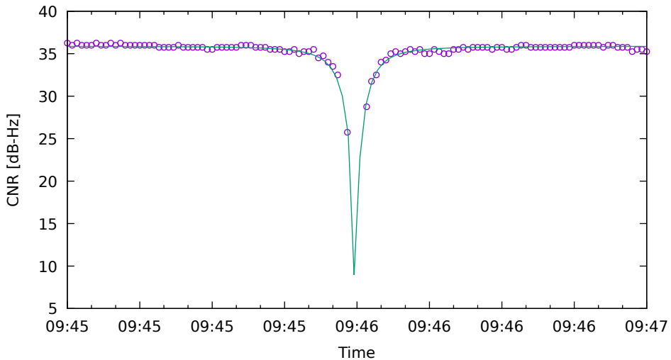
CNR fit for R01 on XiaomiMi8 - drive 4 (DOY263)
