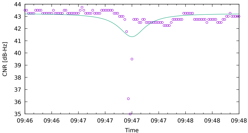
CNR fit for R02 on XiaomiMi8 - drive 5 (DOY263)
