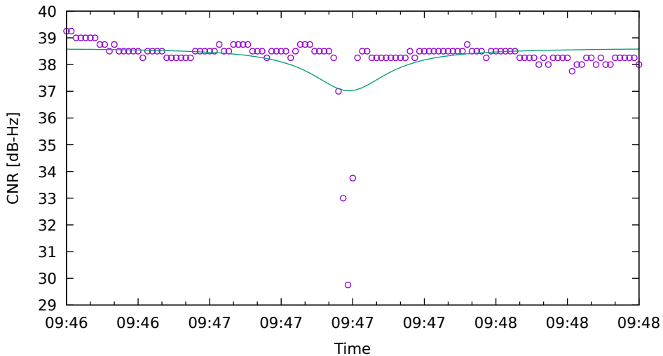
CNR fit for R23 on XiaomiMi8 - drive 5 (DOY263)
