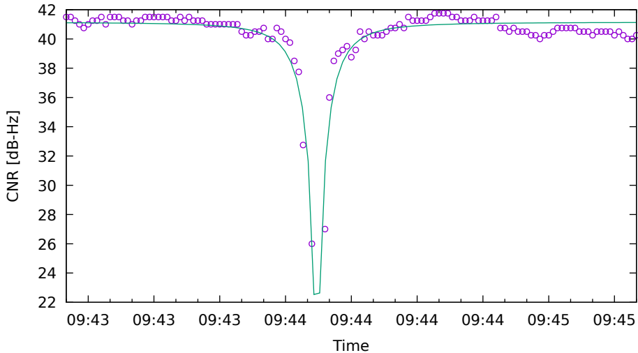
CNR fit for R24 on XiaomiMi8 - drive 3 (DOY263)
