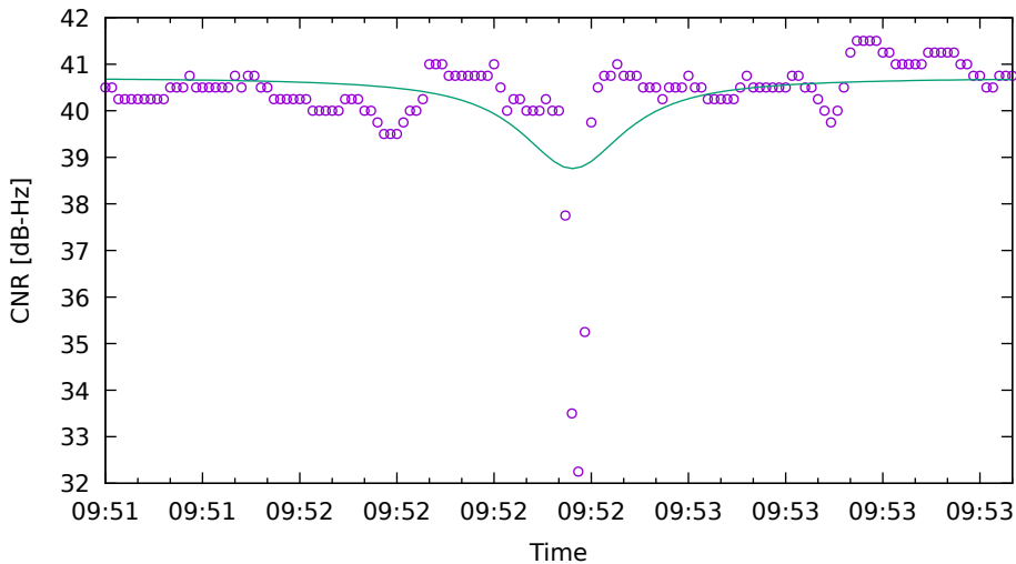
CNR fit for R24 on XiaomiMi8 - drive 8 (DOY263)
