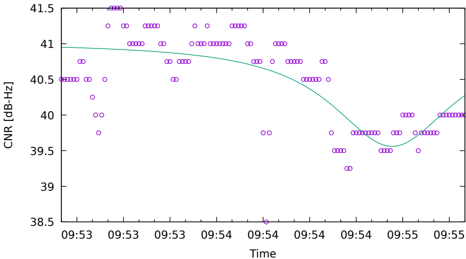
CNR fit for R24 on XiaomiMi8 - drive 9 (DOY263)
