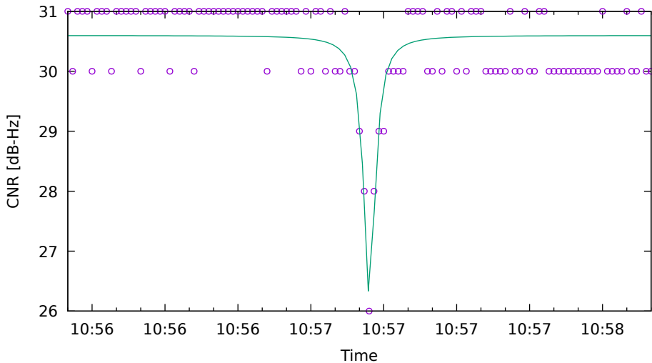
CNR fit for C09 on HuaweiP40 - drive 10 (DOY263)
