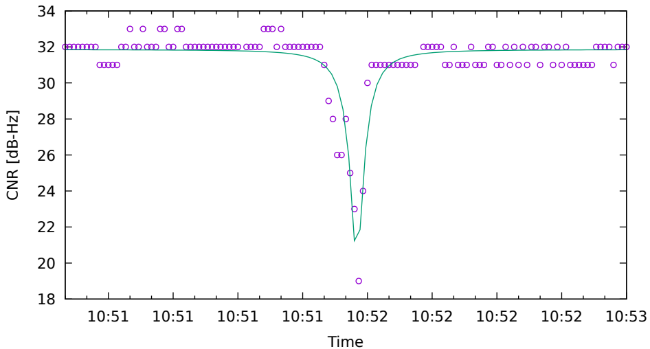
CNR fit for G01 on HuaweiP40 - drive 7 (DOY263)
