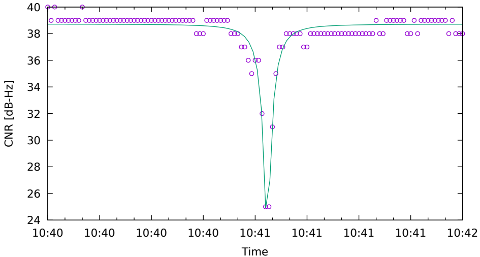
CNR fit for G03 on HuaweiP40 - drive 1 (DOY263)
