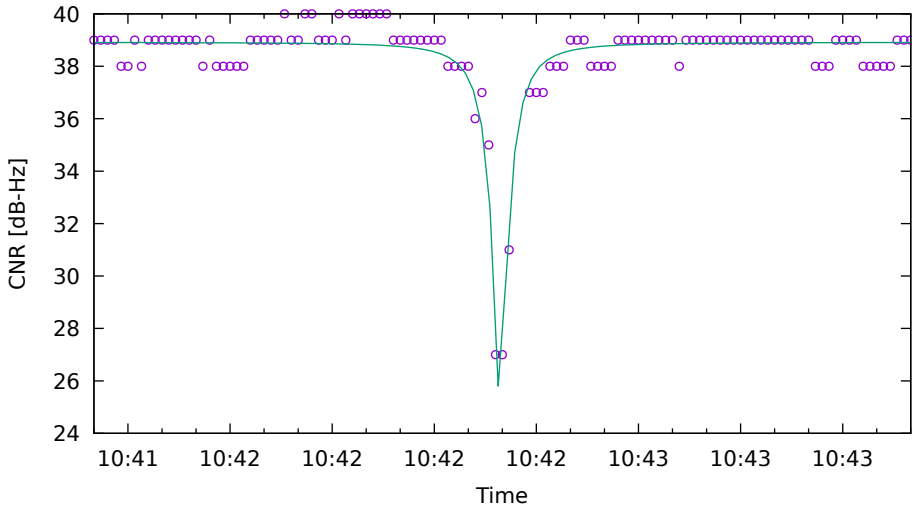
CNR fit for G03 on HuaweiP40 - drive 2 (DOY263)
