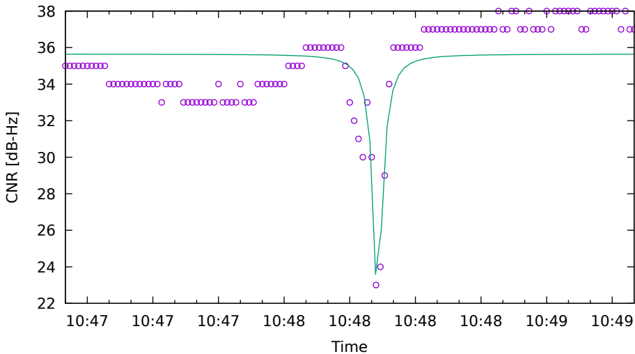
CNR fit for G03 on HuaweiP40 - drive 5 (DOY263)
