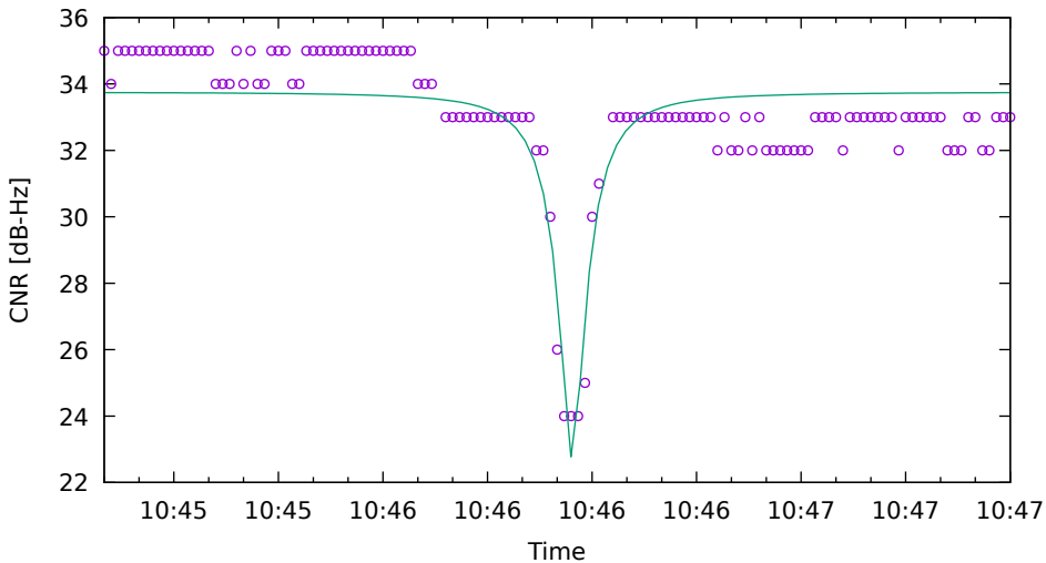
CNR fit for G04 on HuaweiP40 - drive 4 (DOY263)
