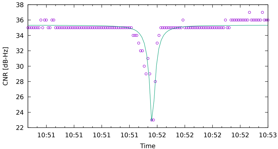
CNR fit for G04 on HuaweiP40 - drive 7 (DOY263)
