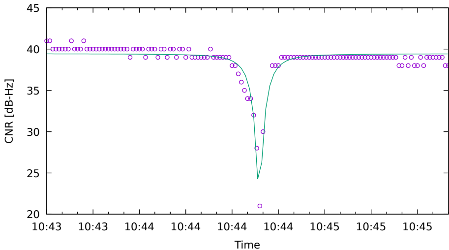
CNR fit for G06 on HuaweiP40 - drive 3 (DOY263)
