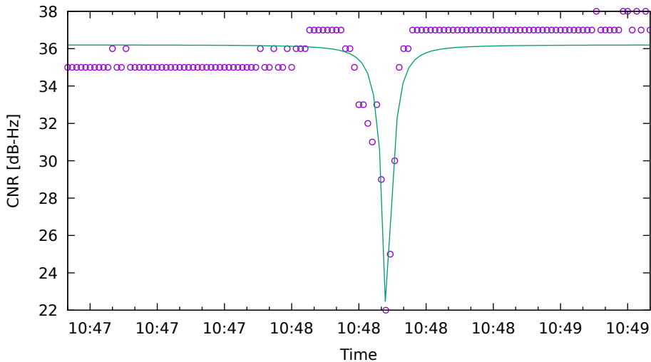
CNR fit for G06 on HuaweiP40 - drive 5 (DOY263)
