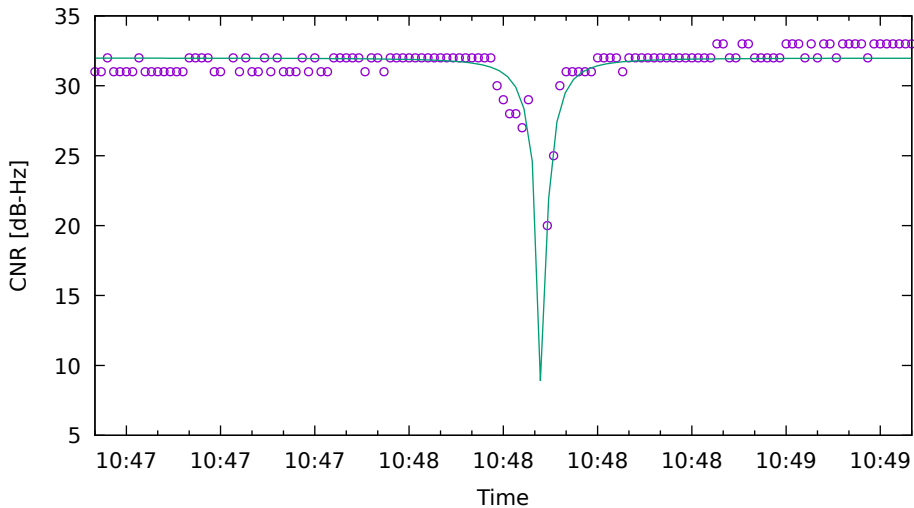
CNR fit for G09 on HuaweiP40 - drive 5 (DOY263)
