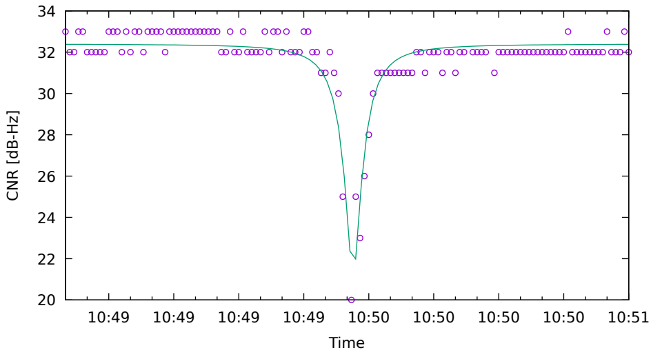
CNR fit for G09 on HuaweiP40 - drive 6 (DOY263)
