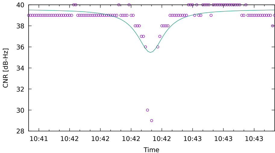
CNR fit for G19 on HuaweiP40 - drive 2 (DOY263)
