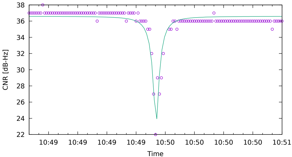
CNR fit for G19 on HuaweiP40 - drive 6 (DOY263)
