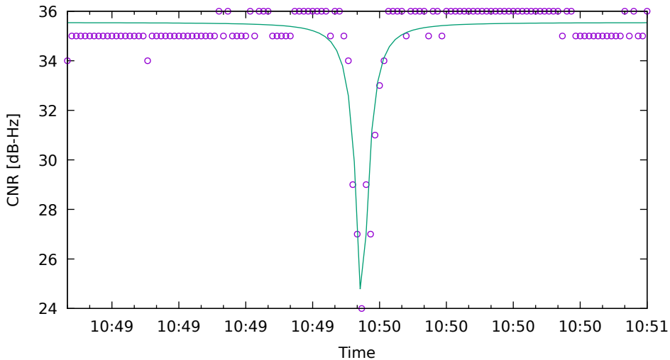
CNR fit for G21 on HuaweiP40 - drive 6 (DOY263)
