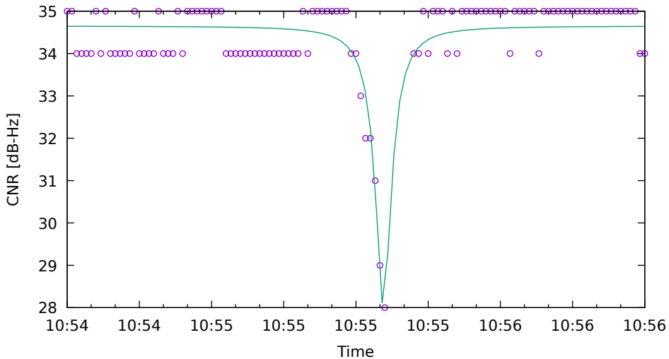
CNR fit for G21 on HuaweiP40 - drive 9 (DOY263)
