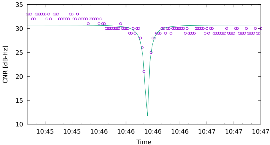
CNR fit for G22 on HuaweiP40 - drive 4 (DOY263)
