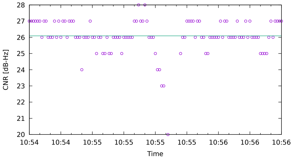
CNR fit for G22 on HuaweiP40 - drive 9 (DOY263)
