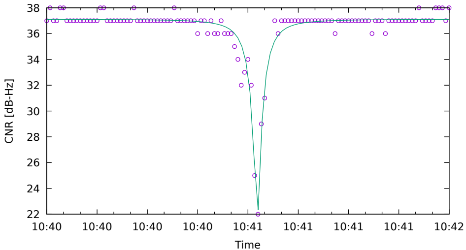
CNR fit for G31 on HuaweiP40 - drive 1 (DOY263)
