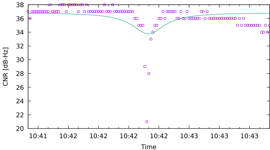
CNR fit for G31 on HuaweiP40 - drive 2 (DOY263)
