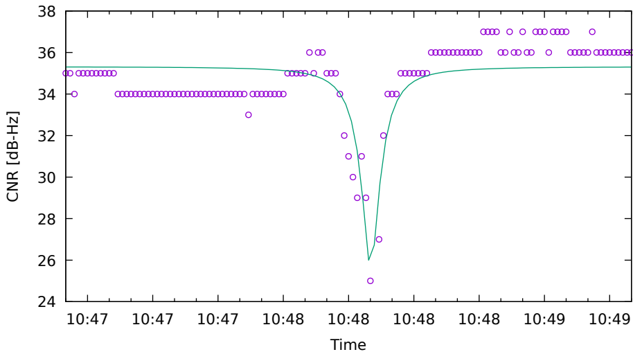
CNR fit for G31 on HuaweiP40 - drive 5 (DOY263)
