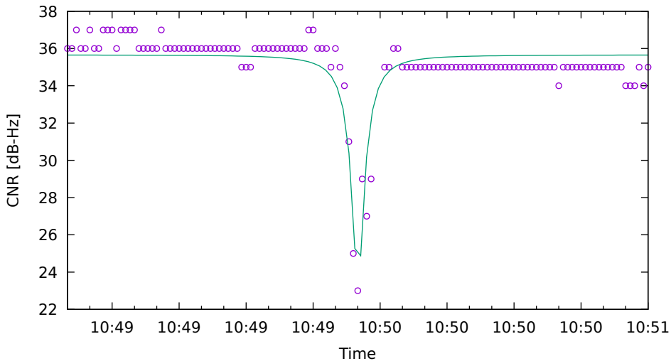
CNR fit for G31 on HuaweiP40 - drive 6 (DOY263)
