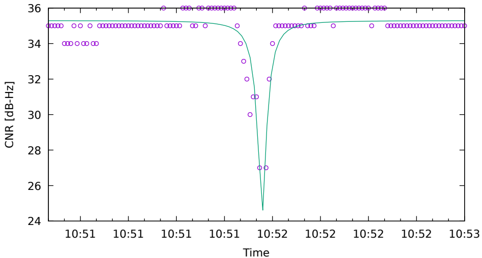
CNR fit for G31 on HuaweiP40 - drive 7 (DOY263)
