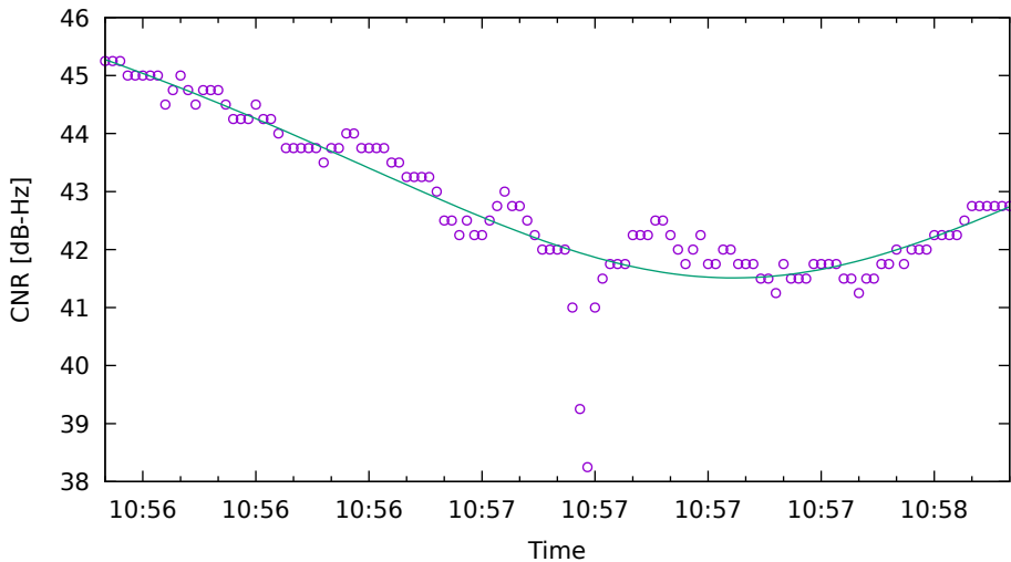
CNR fit for C11 on SamsungS20 - drive 10 (DOY263)
