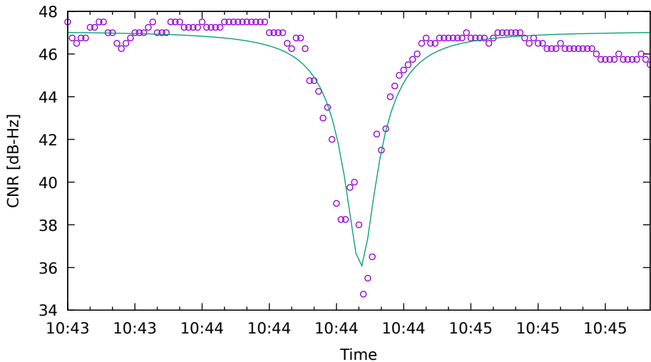
CNR fit for C11 on SamsungS20 - drive 3 (DOY263)
