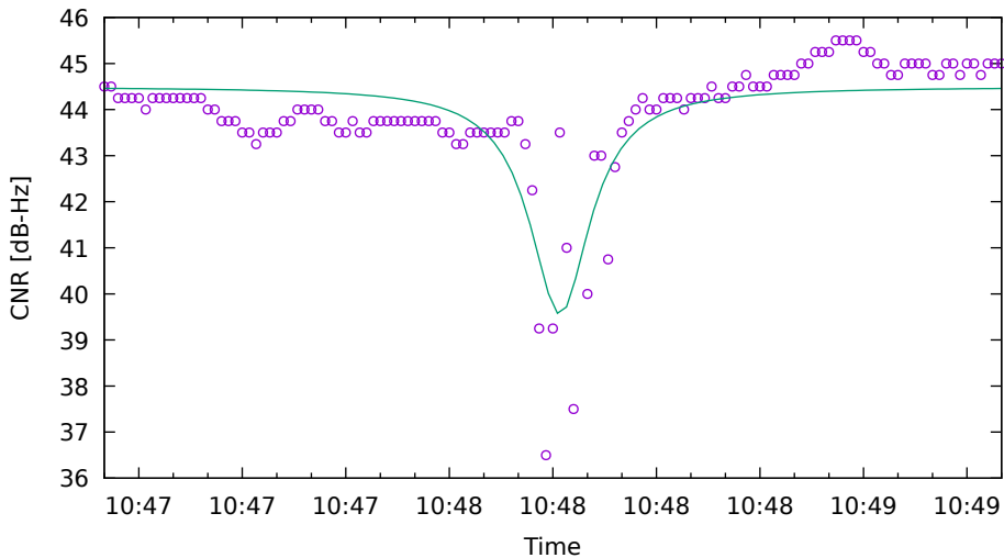
CNR fit for C11 on SamsungS20 - drive 5 (DOY263)
