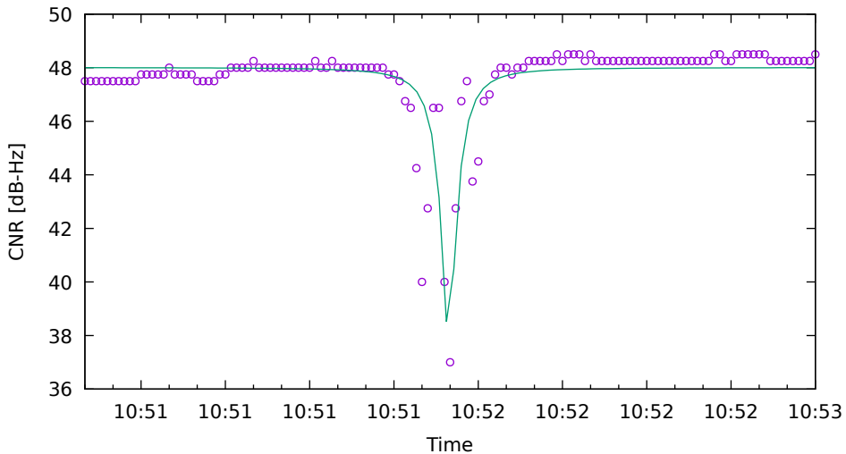
CNR fit for C11 on SamsungS20 - drive 7 (DOY263)
