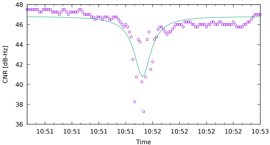
CNR fit for C21 on SamsungS20 - drive 7 (DOY263)
