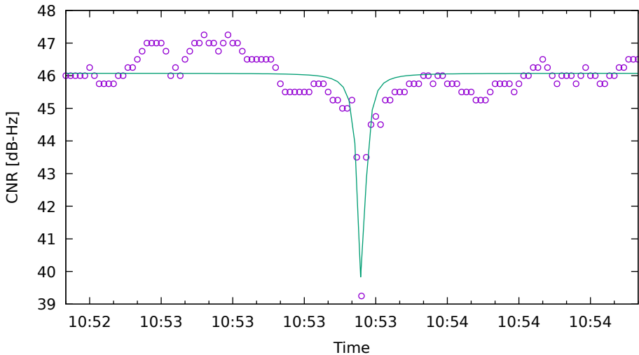
CNR fit for C21 on SamsungS20 - drive 8 (DOY263)
