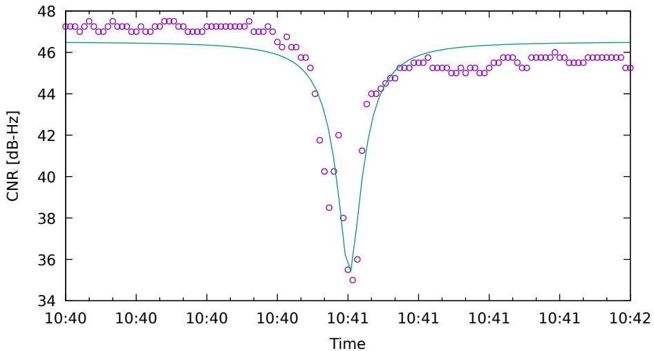
CNR fit for C28 on SamsungS20 - drive 1 (DOY263)
