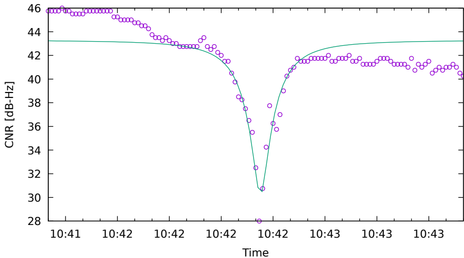
CNR fit for C28 on SamsungS20 - drive 2 (DOY263)
