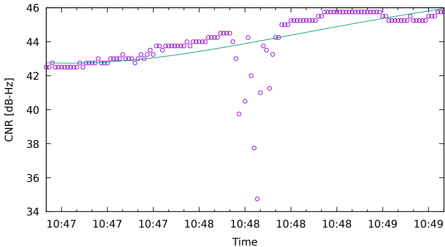
CNR fit for C28 on SamsungS20 - drive 5 (DOY263)
